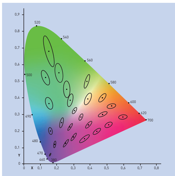
Fig. 6: MacAdam ellipses in the CIE chromaticity diagram
